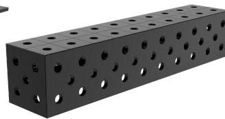
SUORAKULMAINEN U-PALKKI PLUS 1000X200X200 16_50x50_N_019_PLUS 16_100x100_N_019_PLUS 28_100x100_N_019_PLUS
